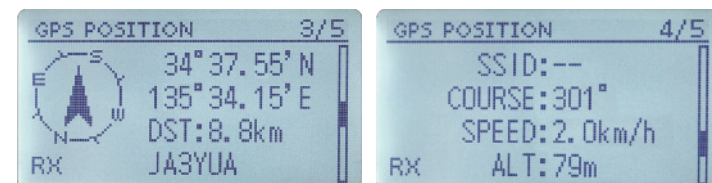
RX (Received station) position information example
